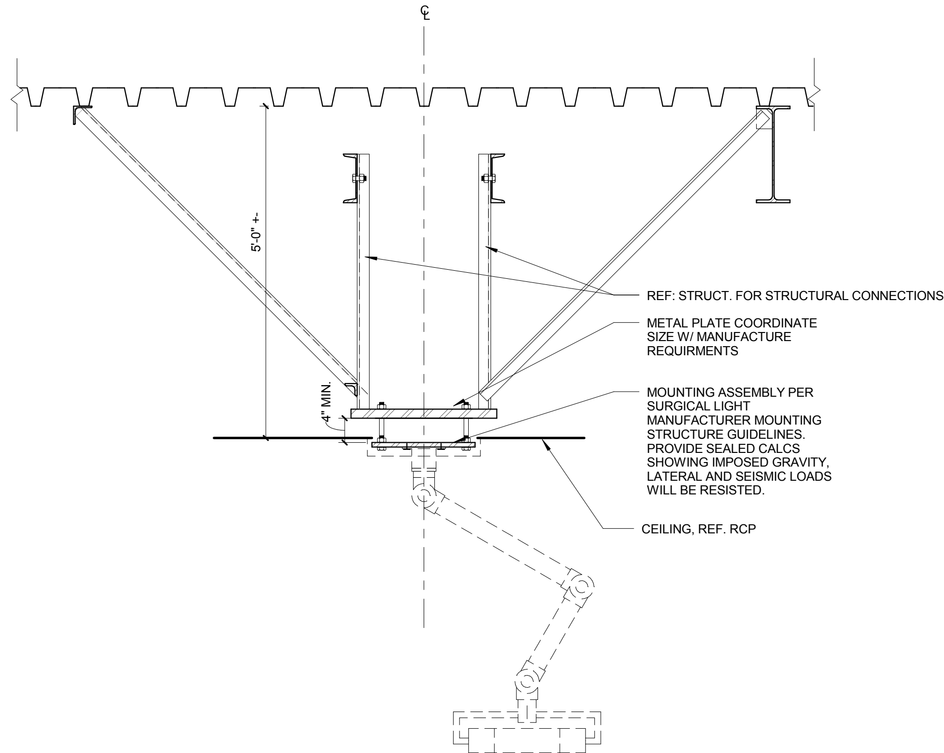
1 SURGERY LIGHT SUPPORT 3/4" = 1'-0"
